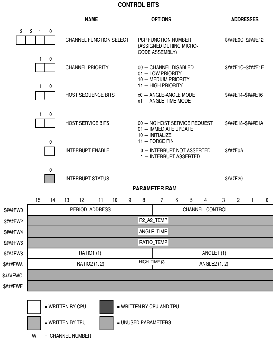
Figure A-5 shows the host interface areas and parameter RAM for the PSP function.
