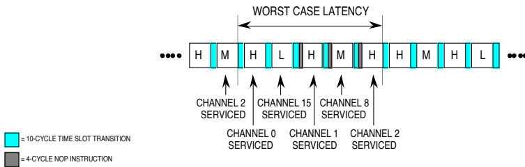
Figure C-11 Worst-Case Latency for Channel 2
