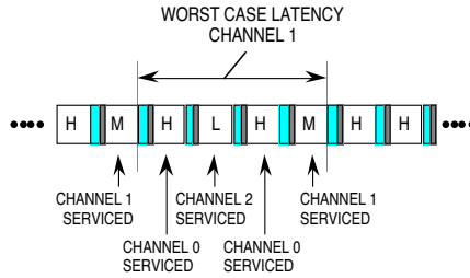
Figure C-7 Next Servicing for Channel 1
