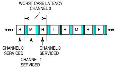
Figure C-6 Next Servicing for Channel 0
