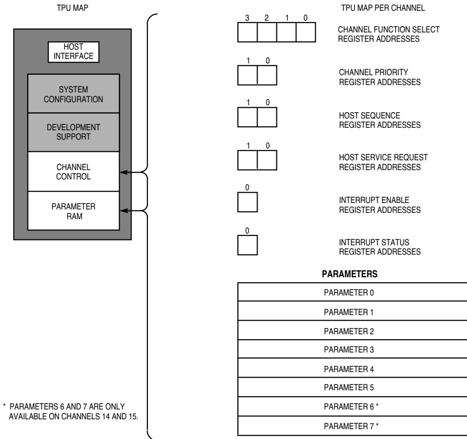
Figure 2-5 Channel Control and Parameter RAM Configuration
