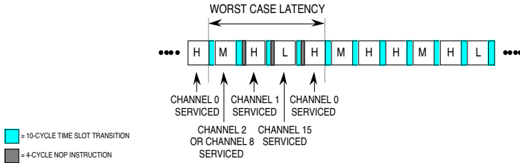
Figure C-10 Worst-Case Latency for Channel 0 (Second Try)
